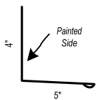
4 Sidewall Trim
